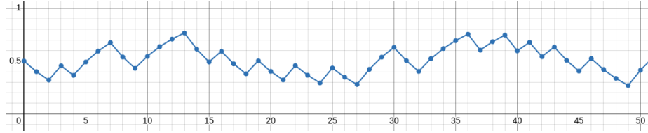
Figure 1: A sequence of 50 mastery levels generated from an answer sequence whose samples are each 1 or 0 with equal probability. Note how consecutive correct or incorrect answers yield diminishing returns.
